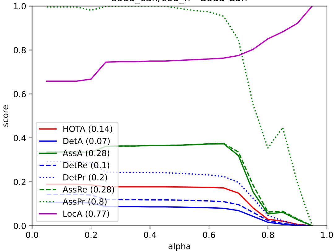
soda_can/cou_n - Soda Can
